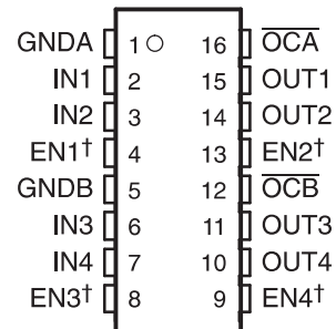
TPS2095, TPS2096 AND TPS2097 D PACKAGE
